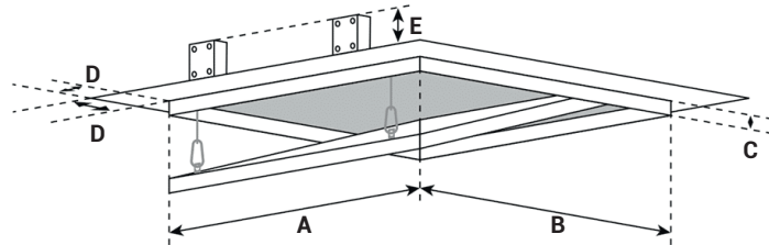
STANDARD DIMENSIONS WITH 1/2" DRYWALL INLAY:
