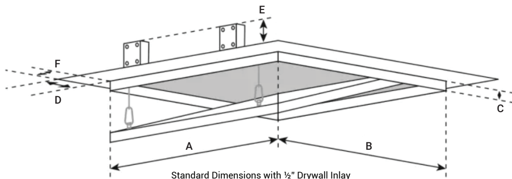
Standard Dimensions with 1/2" Drywall Inlay
