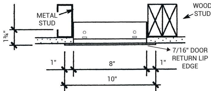
SECTION DETAILS
