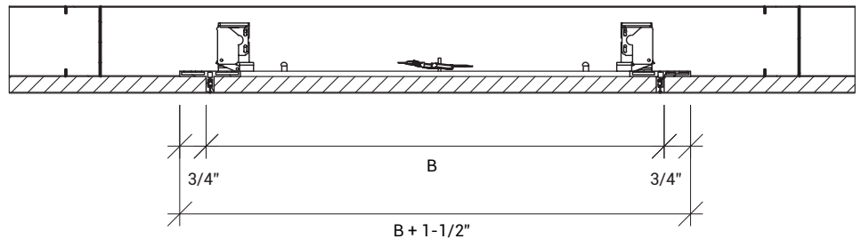
SECTION DETAIL
