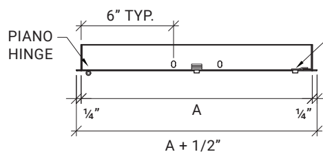
SECTION DETAIL
