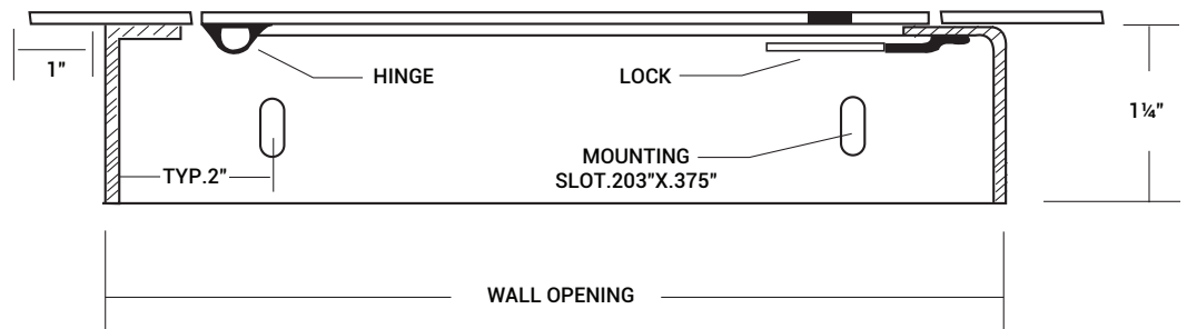
SECTION DETAIL
