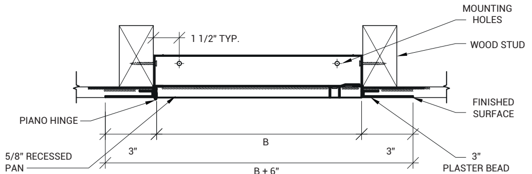
SECTION DETAIL
