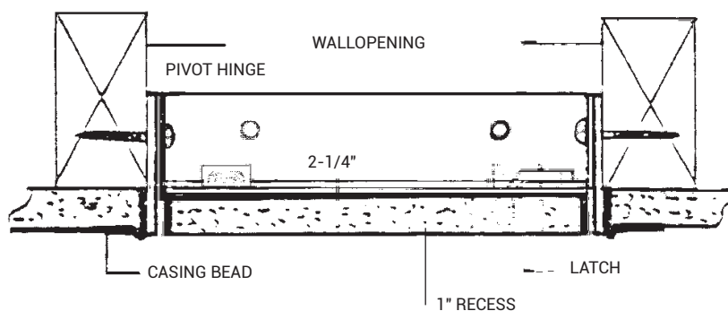
SECTION DETAIL
