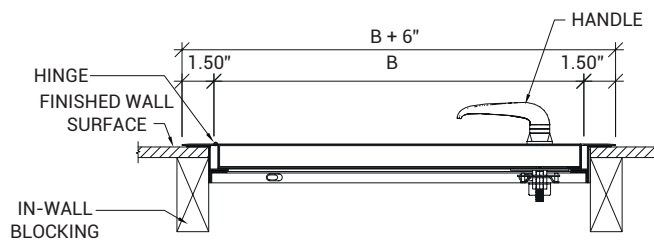
SECTION DETAIL
