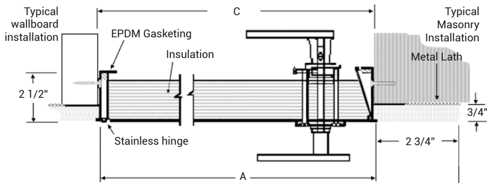
H4 Inside Latch Removable Flush Locking Handle
