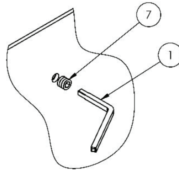
LATCH DETAIL
