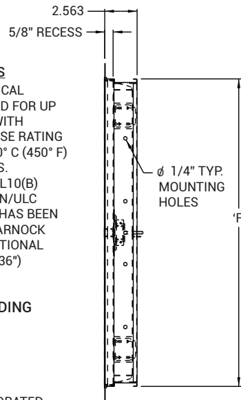
DOOR AND FRAME 22 GA. (.034) SATIN COAT STEEL
